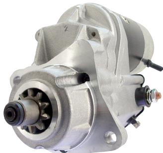
19962N 2.5kw, CW, 10T
